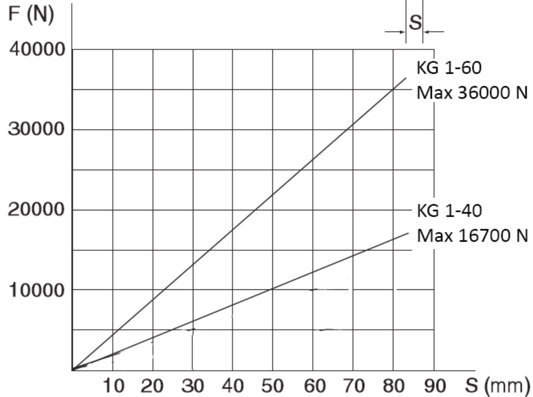
SHEAR LOAD Static Spring Rate
