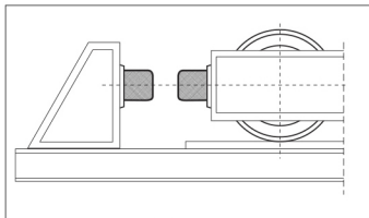
Fig. 2. Traverse crane with 2 buffers connected in series.
