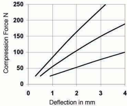
elasto-Flex-Elements Type 60
