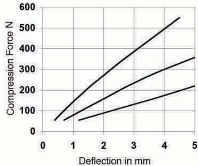
elasto-Flex-Elements Type 90
