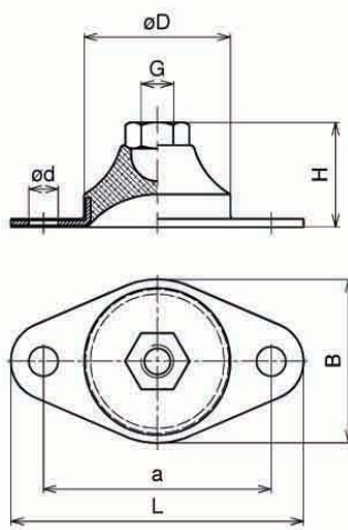
elasto-Flex-Elements Type 90
