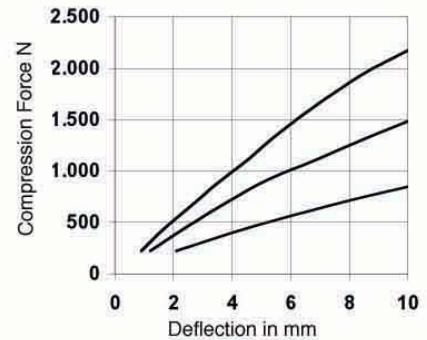
elasto-Flex-Elements Type 140
